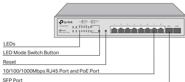
Figure 1-1 Front Panel of T1500G-10MPS
