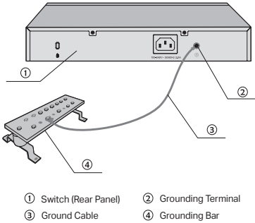
Figure 3-1 Connecting to the Grounding Bar
